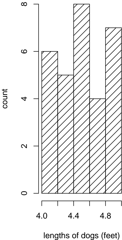
Histogram of len1
